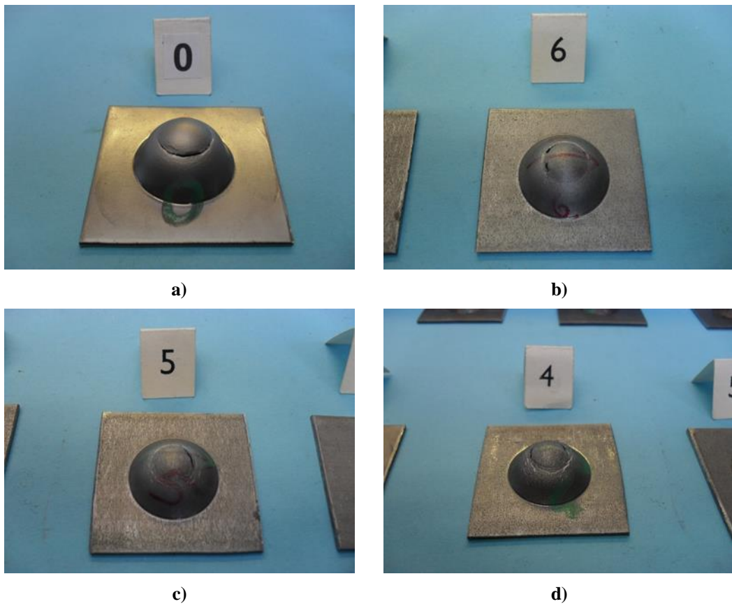
Fig. 9 Crack of the steel DC01 after ERICHSEN test: a) initial state, b) after 2 nd , c) 4 th , d) 6 th pass by DRECE
