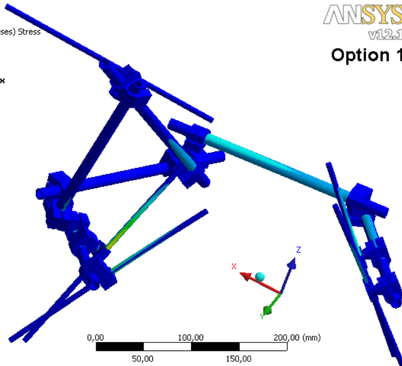
Fig. 6 “Option 1” - FE modelling of external fixator for pelvis and acetabulum (equivalent stresses for tensile loading 100 N)
