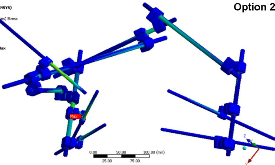
Fig. 7 “Option 2” - FE modelling of external fixator for pelvis and acetabulum (equivalent stresses for tensile loading 100 N)
