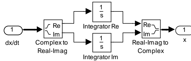
Fig. 6 Integration of complex signals.
