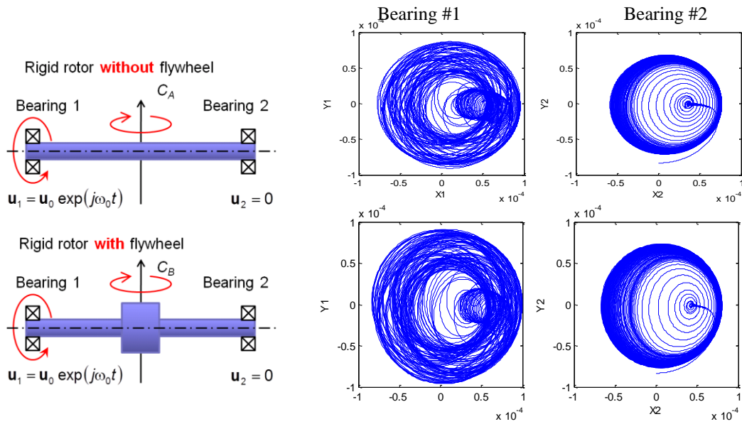
Fig. 8 Effect of circulation of the bearing bushing #1 on movement of the journal in the bearing #2
