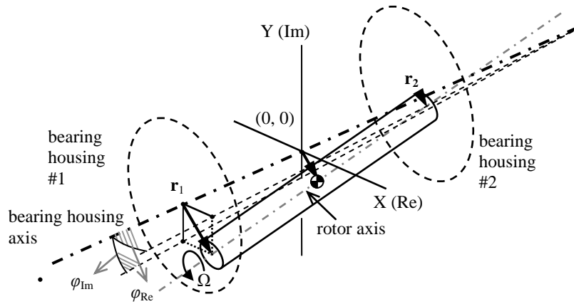
Fig. 5 Rotor inclinations.
