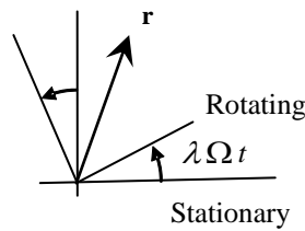
Fig. 4 Transformation of rotating coordinates to stationary coordinates.
