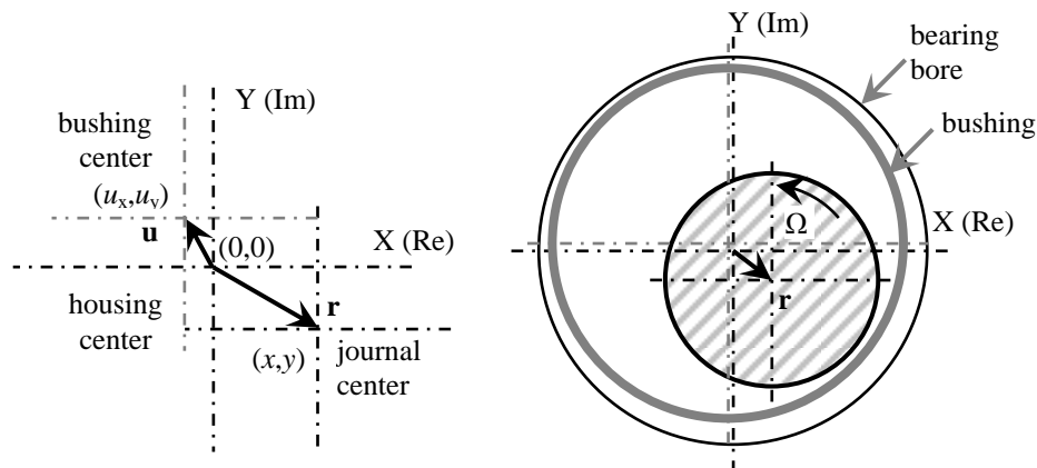
Fig. 2 Coordinate system.
