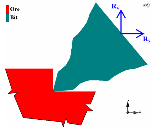
Fig. 20 Reaction Forces in the Bit.
