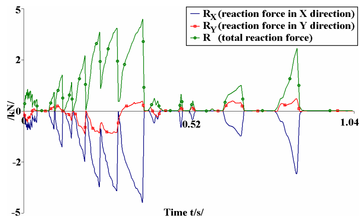
Fig. 21 Reaction Forces in the Bit.
