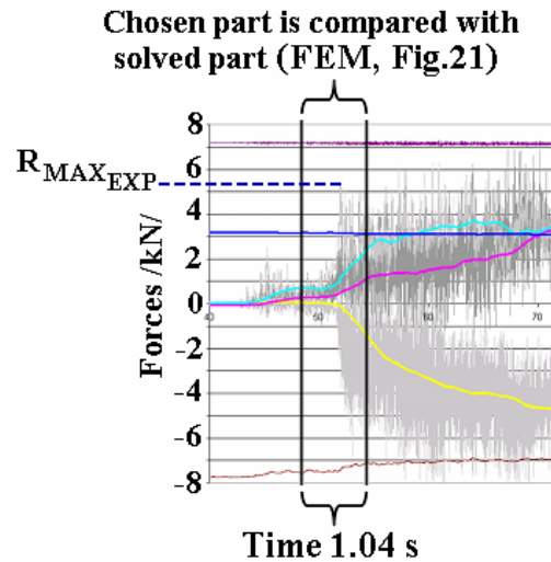
Fig. 22 Experimental Measurements (Forces and Other Acquired Quantities) and its Comparison with the FE Solution.
