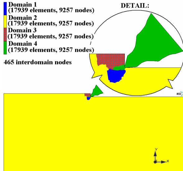
Fig. 8 Domain Decomposition Method Applied for 4×CPU.
