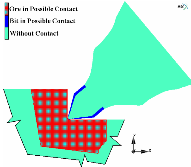
Fig. 5 Boundary Conditions (Mechanical Contacts).
