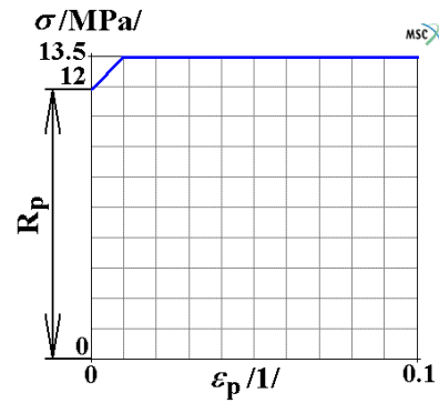
Fig. 7 Relationship between Stress and Plastic Strain for Ore.
