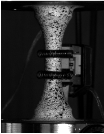
Fig. 4 Sprayed specimen
